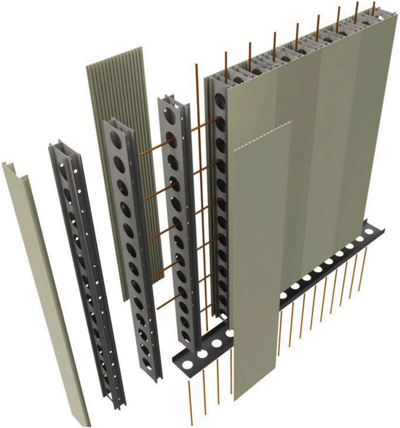
FIGURE 2 PERMAFORM CONSTRUCTION
